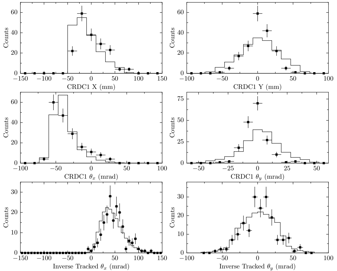
Figure 4.24: Comparison of simulation to data for ^{18}\text{C} reaction fragments.
