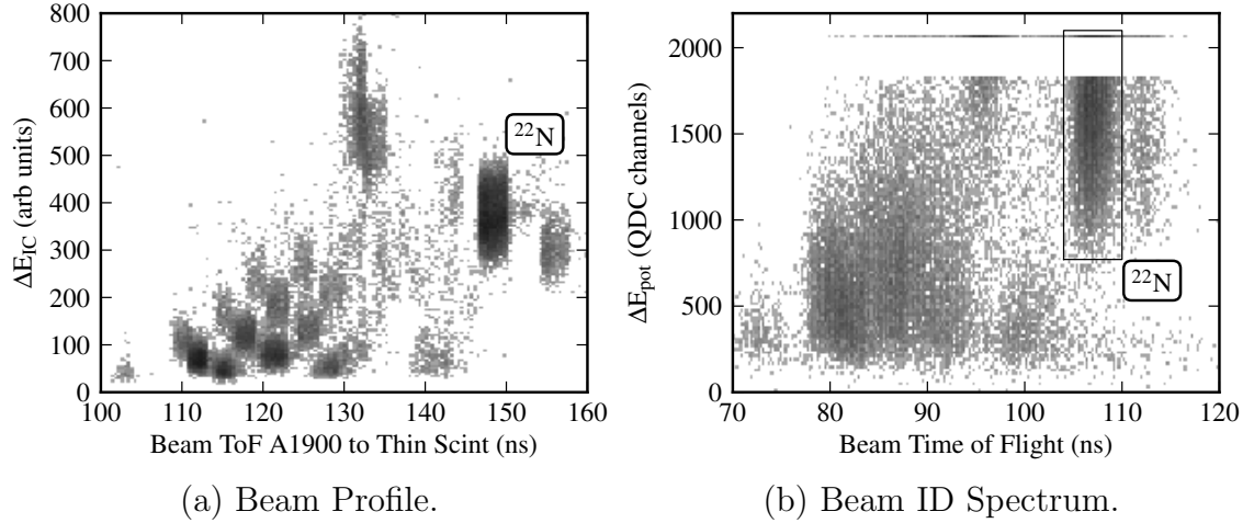
Figure 4.14: Beam profile and beam ID spectra.
