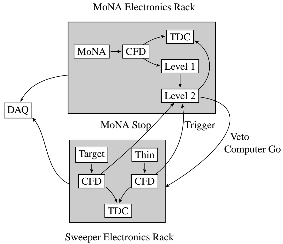
Figure 3.5: Trigger logic diagram.
