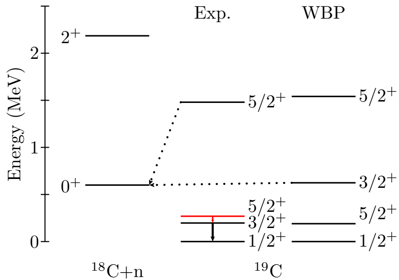
Figure 2.5: Experimental level scheme for ^{19}\text{C} based on results from [12, 16, 17].
