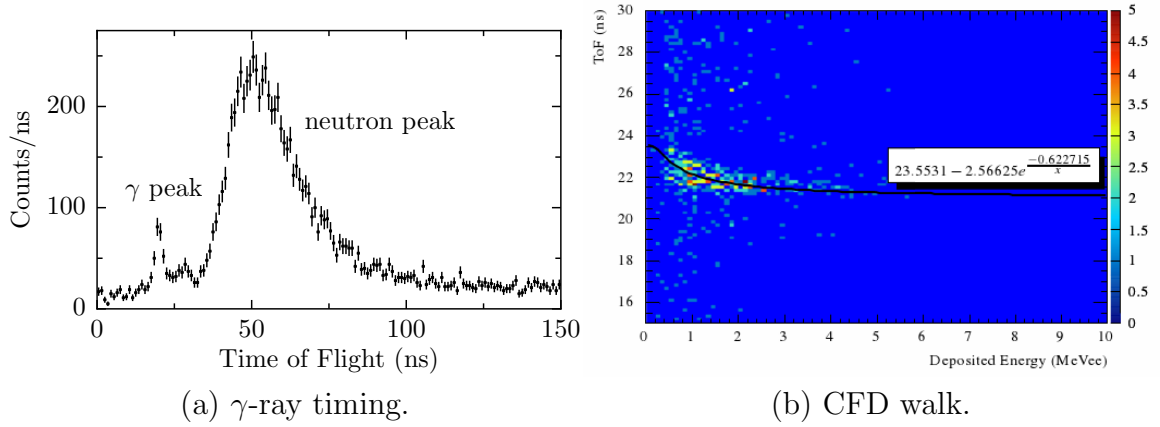
Figure 4.13: \gamma -ray timing and CFD walk corrections.
