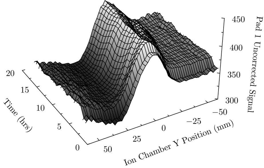
Figure 4.11: Position and time dependence of pad 1.
