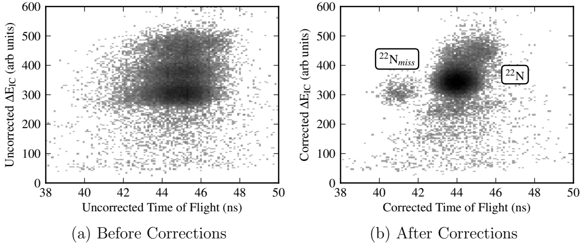
Figure 4.12: Resolution comparison of uncorrected ion chamber and physical target scintillator (a) to corrected ion chamber and virtual target scintillator (b). Element separation is only possible in (b), and the improved timing resolution allows clean separation of ^{22}\text{N} missing the target.
