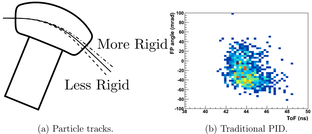
Figure 4.16: Particle tracks for different carbon isotopes through the sweeper magnet (a), and a traditional particle ID attempt from plotting dispersive angle vs. time of flight (b). Correlations between angle, position, and time of flight preclude such a treatment (see text).
