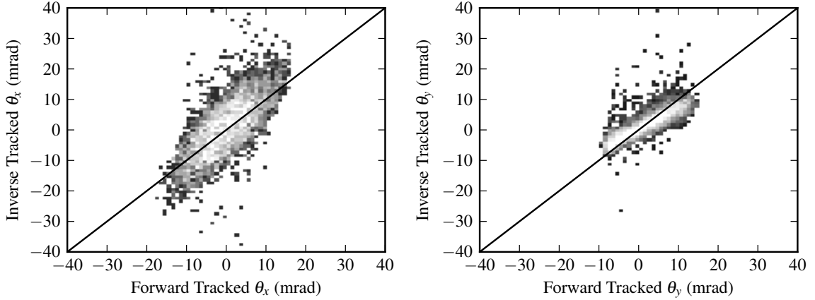
Figure 4.21: Consistency check for magnetic field map transformations showing reasonable agreement between the forward and inverse tracking processes.
