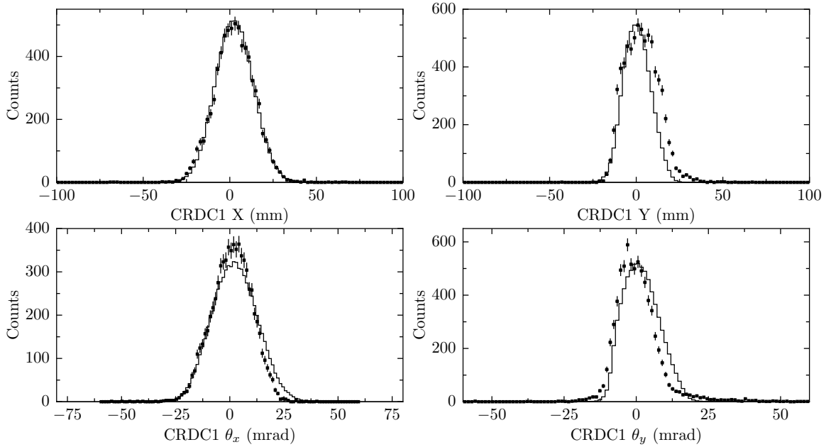
Figure 4.22: Comparison of simulation to data for ^{22}\text{N} reaction fragments.
