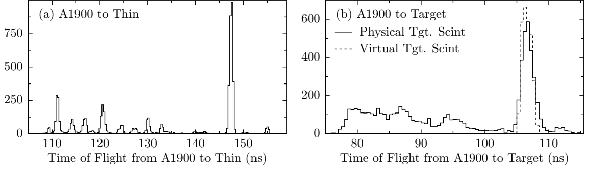
Figure 4.3: Resolution comparison between the target chamber and thin scintillators for a no-target run. The beam particle peaks in the spectrum utilizing the target chamber scintillator (right solid) is a factor of 2.5 wider than the corresponding peaks in the time spectrum utilizing the thin scintillator (left) despite the A1900 to thin flight path being longer. This widening is entirely due to resolution effects. The virtual target scintillator (right dashed) improves the resolution by \sim 20\% .
