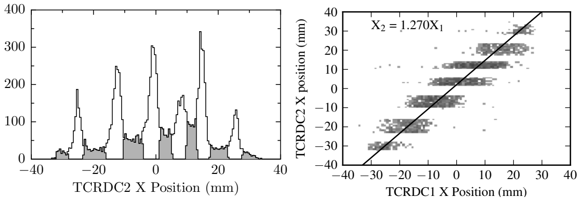
Figure 4.8: TCRDC2 charge collection issue (left) and the correlation between TCRDC positions used to replace the physical device’s x position information.
