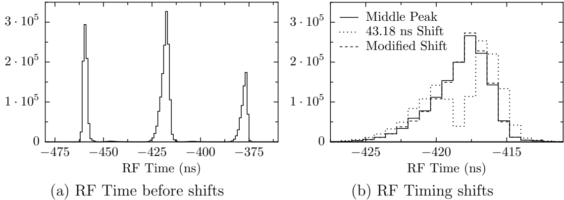
Figure 4.2: The downscaled RF timing signal showing up as three peaks in an uncorrected time spectrum (a). In (b), the 43.18 ns shift corresponding to the cyclotron frequency does not match the middle RF peak, while adjusting the shift parameters slightly (see text) results in good agreement.
