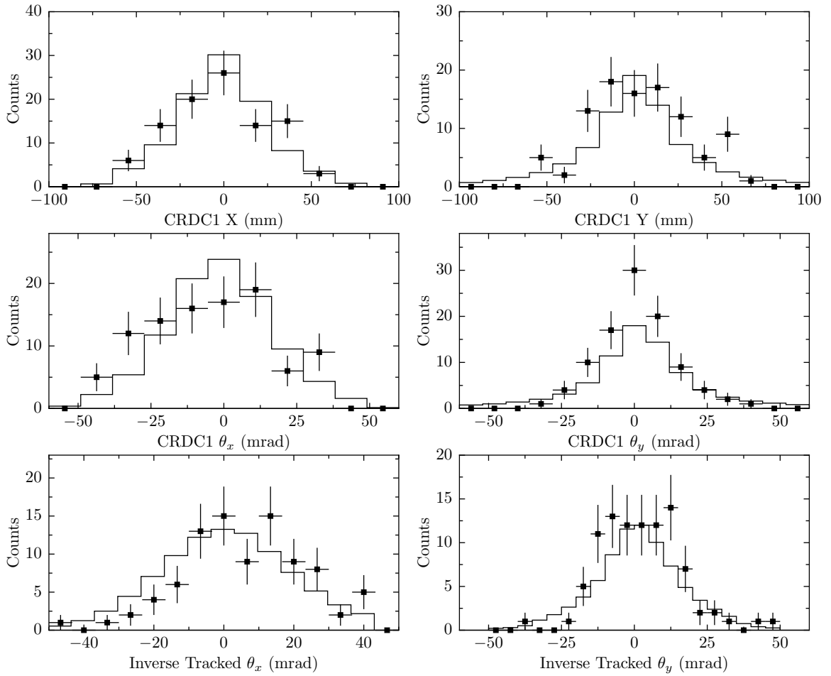
Figure 4.23: Comparison of simulation to data for ^{20}\text{C} reaction fragments.
