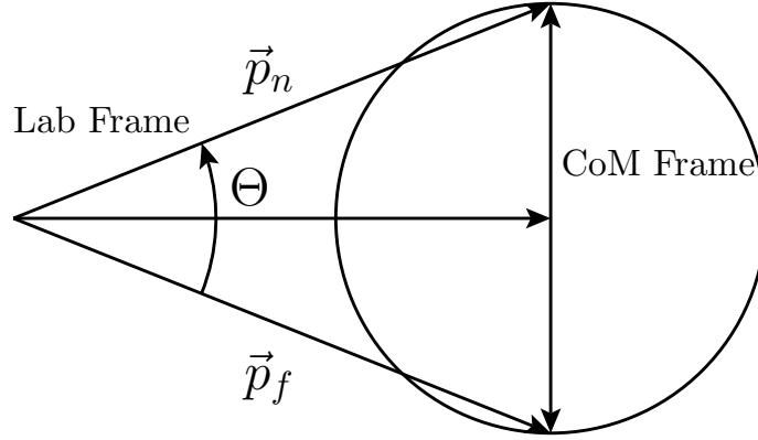
Figure 3.1: Neutron evaporation schematic.
