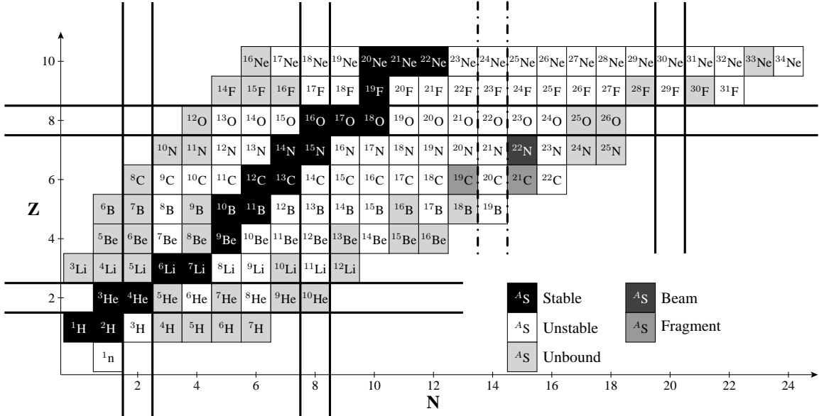
Figure 1.2: Chart of nuclides with “magic numbers” illustrated and this work’s beam and reaction products of interest indicated.
