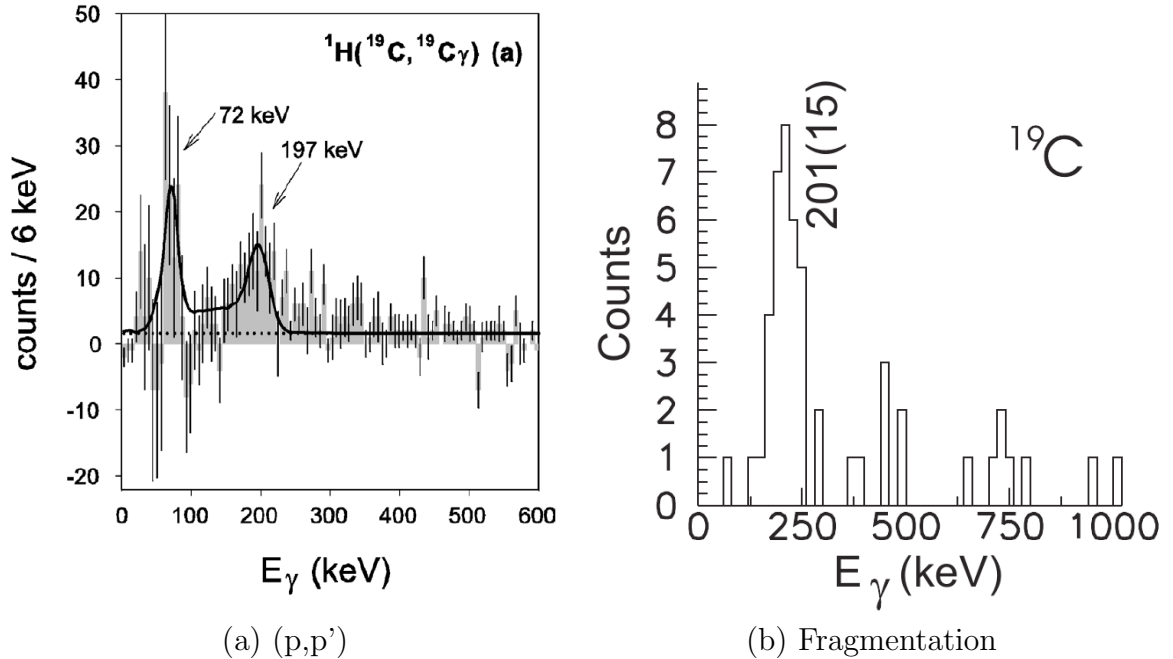
Figure 2.3: Resulting \gamma -ray spectrum for bound excited states in ^{19}\text{C} from [16] and [12].
