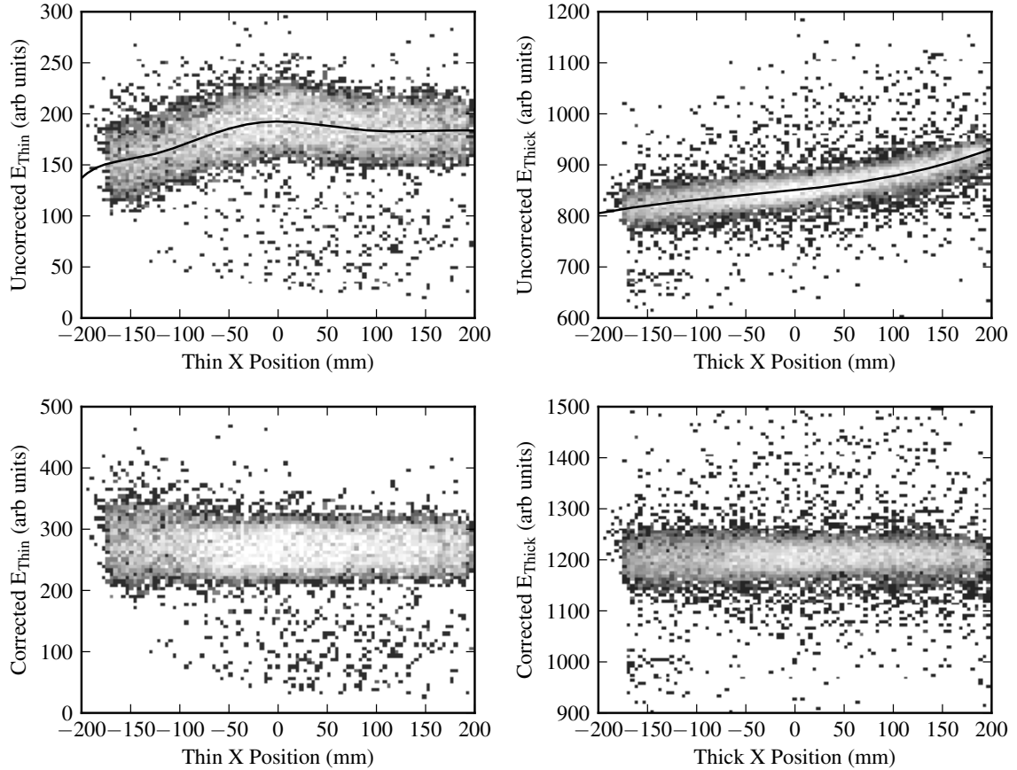
Figure 4.9: Thin (top left) and thick (top right) response as a function of x position and the corresponding correction curves. The bottom panels show the correction taking effect for both scintillators, which results in a flattened spectrum with position correlations removed.
