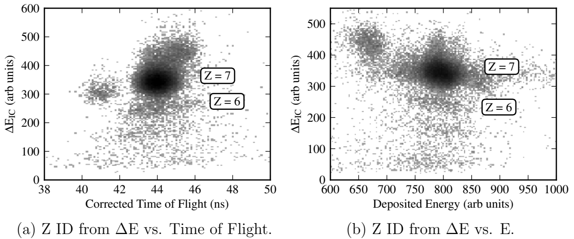
Figure 4.15: Element separation by two different methods - \Delta E vs. Time of Flight and \Delta E vs. E . Both methods are combined to reduce contamination from unreacted beam.
