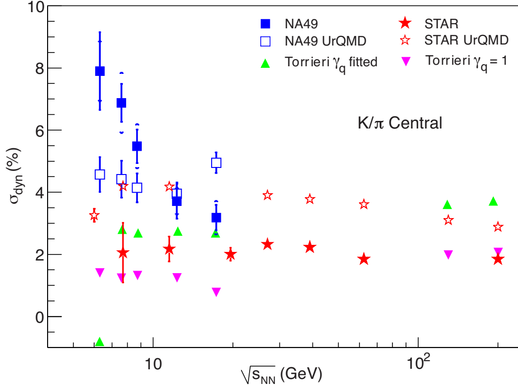
Figure 5.4: Energy dependence of \sigma_{\text{dyn},K\pi} results. STAR results (red stars) are from Au+Au collisions, 0-5% centrality, only statistical errors are shown, while NA49 results (blue squares) are from Pb+Pb collisions, 0-3.5% centrality, both statistical and systematical error are shown.
