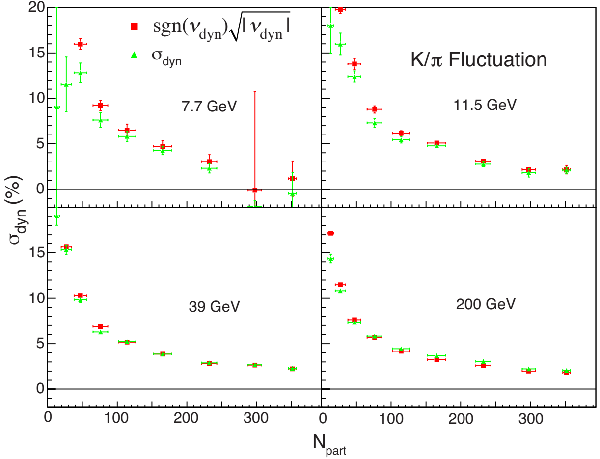
Figure 5.16: Centrality dependence of \text{sgn}(\nu_{\text{dyn}})\sqrt{|\nu_{\text{dyn}}|} and \sigma_{\text{dyn},K\pi} results from Au+Au collisions at \sqrt{s_{\text{NN}}} = 7.7, 11.5, 39 and 200 GeV.
