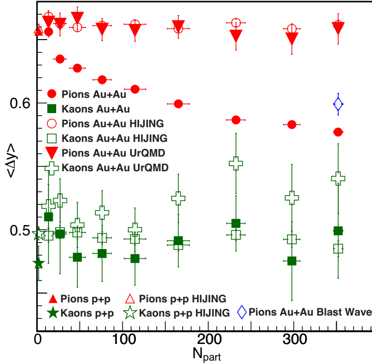
Figure 6.18: The balance function widths for identified charged pions and charged kaons from Au+Au collisions at \sqrt{s_{\text{NN}}} = 200 GeV and p + p collisions at \sqrt{s} = 200 GeV. Filtered HIJING calculations are shown for the same systems. Filtered UrQMD calculations are shown for Au+Au. Also shown is the width of the balance function for pions predicted by the blast-wave model of Ref. [61].
