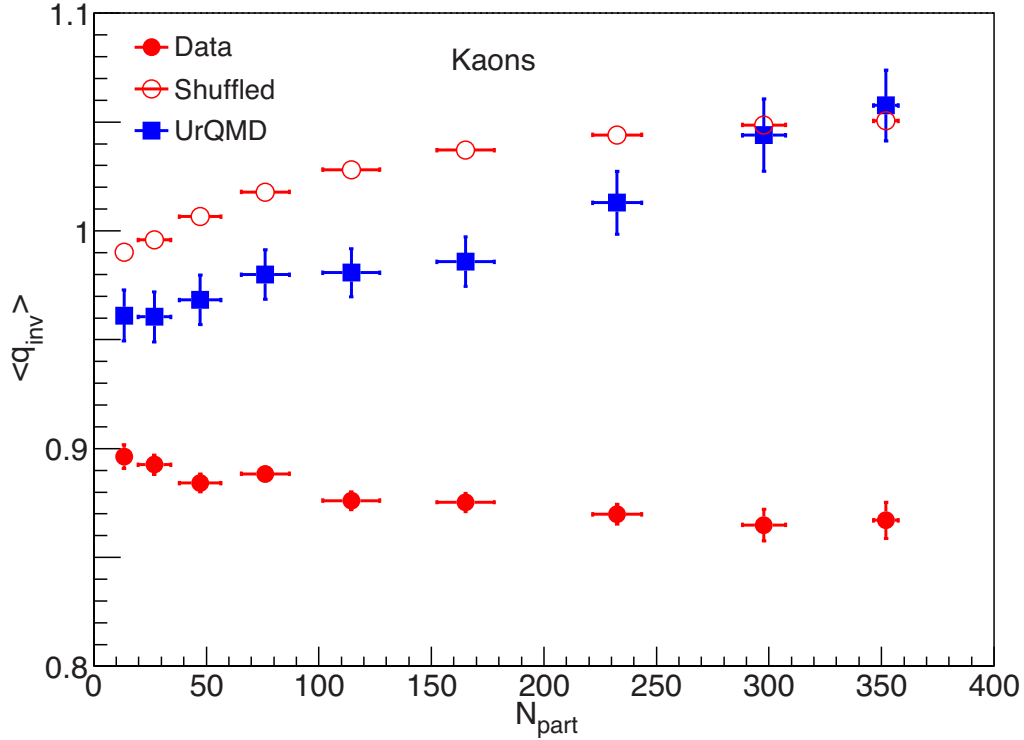
Figure 6.42: Centrality dependence of the balance function widths of q_{inv} for identified charged kaons from Au+Au collisions at \sqrt{s_{NN}} = 200 GeV.
