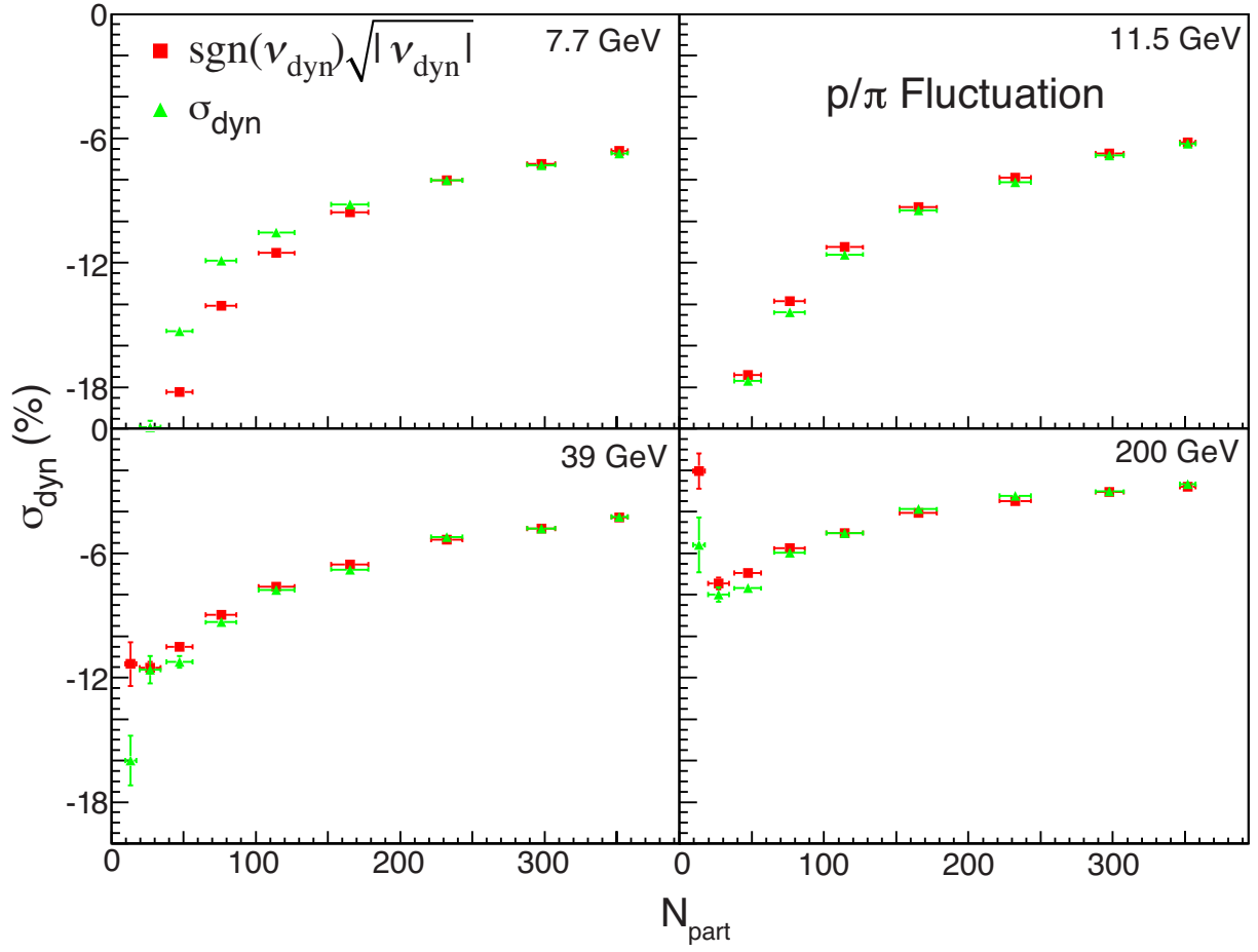
Figure 5.17: Centrality dependence of \text{sgn}(v_{\text{dyn}})\sqrt{|v_{\text{dyn},p\pi}|} and \sigma_{\text{dyn},p\pi} results from Au+Au collisions at \sqrt{s_{\text{NN}}} = 7.7, 11.5, 39 and 200 GeV.
