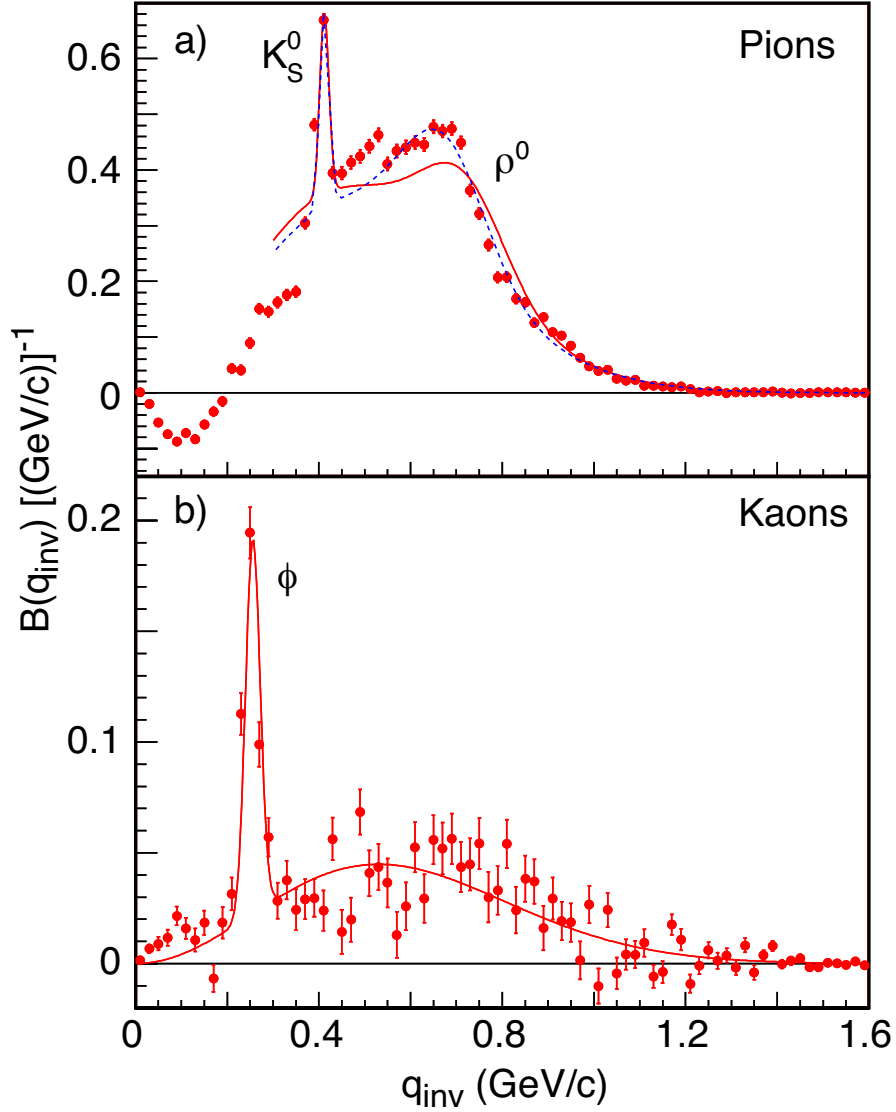
Figure 6.9: The balance function in terms of q_{\text{inv}} for charged pion pairs [part a)] and charged kaon pairs [part b)] from p + p collisions at \sqrt{s} = 200 \text{ GeV} integrated over all multiplicities. Solid curves correspond to a thermal distribution (Equation 6.1) plus K_S^0 and \rho^0 decay for pions and \phi decay for kaons. The dashed curve for pions represents a fit to a thermal distribution (Equation 6.1) plus K_S^0 decay and \rho^0 decay, with the \rho^0 mass shifted down by 0.04 \text{ GeV}/c^2 .
