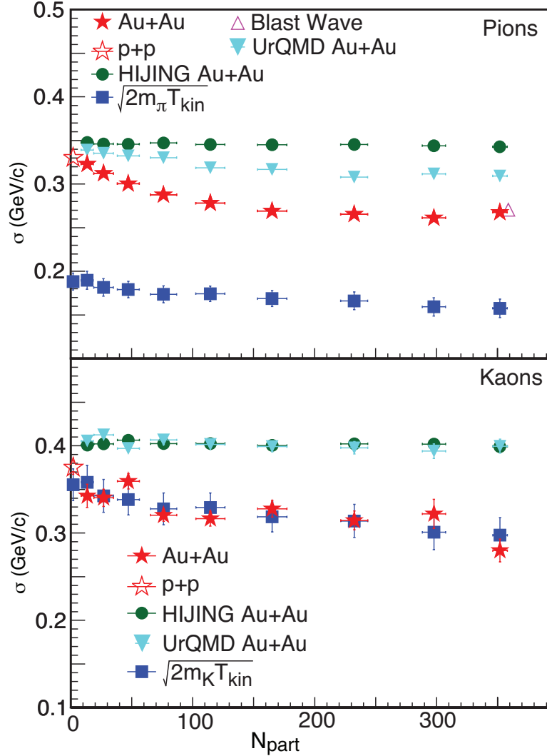
Figure 6.19: The balance function width \sigma extracted from B(q_{\text{inv}}) for identified charged pions and kaons from Au+Au collisions at \sqrt{s_{\text{NN}}} = 200 GeV and p + p collisions at \sqrt{s} = 200 GeV using a thermal fit (Equation 6.1) where \sigma is the width. Filtered HIJING and UrQMD calculations are shown for pions and kaons from Au+Au collisions at \sqrt{s_{\text{NN}}} = 200 GeV. Values are shown for \sqrt{2mT_{\text{kin}}} from Au+Au collisions, where m is the mass of a pion or a kaon, and T_{\text{kin}} is calculated from identified particle spectra [65]. The width predicted by the blast-wave model of Ref. [61] is also shown for pions.
