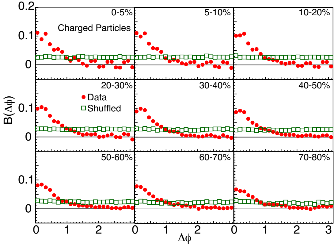
Figure 6.14: The balance function in terms of \Delta\phi for all charged particles with 1.0 < p_t < 10.0 GeV/ c from Au+Au collisions at \sqrt{s_{\text{NN}}} = 200 GeV in nine centrality bins. The closed circles represent the real data minus the mixed events.
