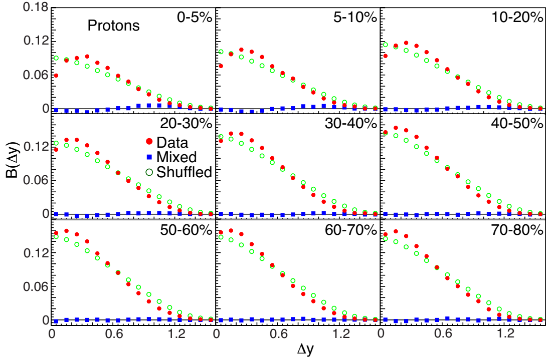
Figure 6.37: The balance function in terms of \Delta y for identified charged proton pairs from STAR Run 10 Au+Au collisions at \sqrt{s_{NN}} = 200 GeV for nine centrality bins.
