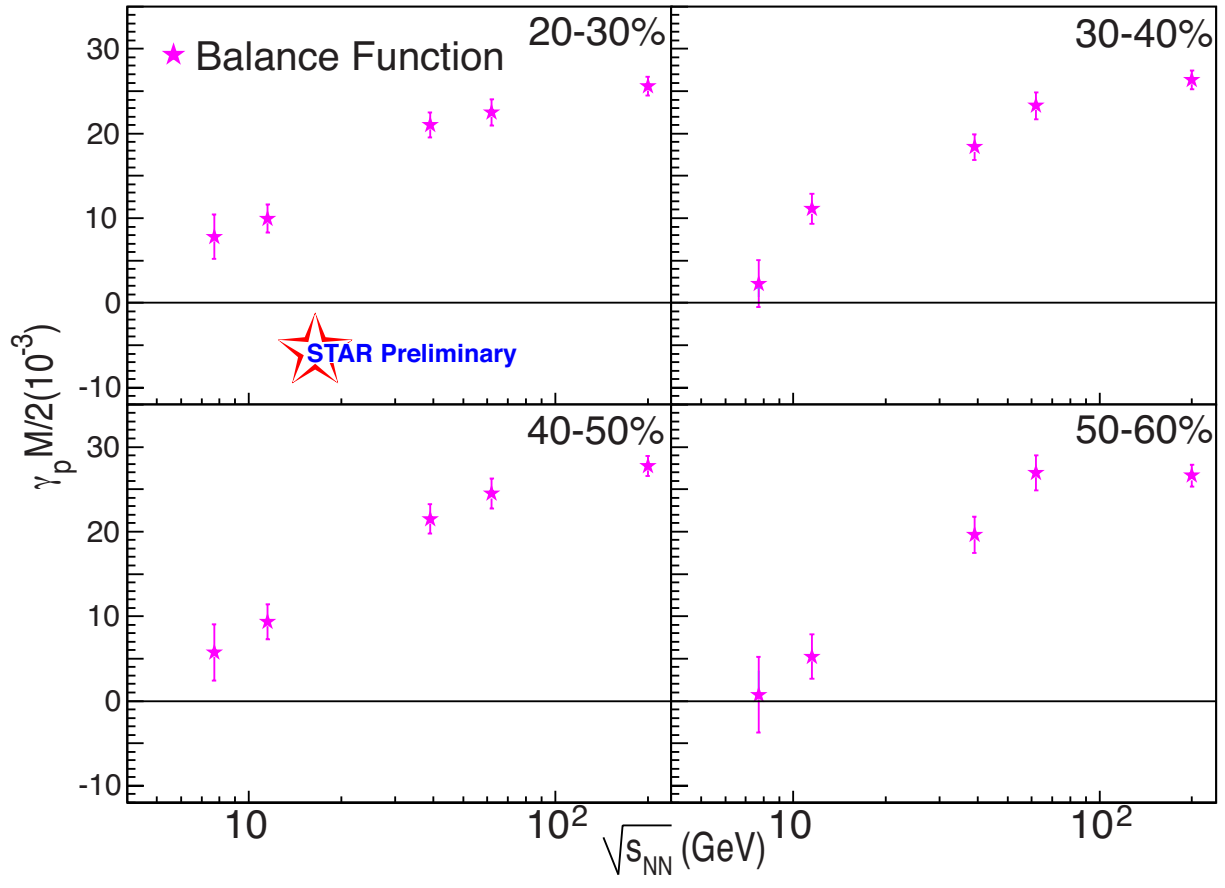
Figure 6.32: The beam energy dependence of balance function. Four centralities are shown here.
