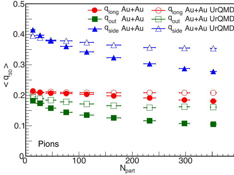
Figure 6.20: The widths for the balance functions for pions in terms of q_{\text{long}} , q_{\text{out}} , and q_{\text{side}} compared with UrQMD calculations.
