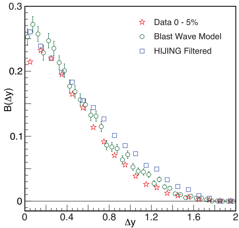
Figure 6.15: The balance function in terms of \Delta y for charged pions from central collisions of Au+Au at \sqrt{s_{NN}} = 200 GeV compared with predictions from the blast-wave model from Ref. [61] and filtered HIJING calculations taking into account acceptance and efficiency.
