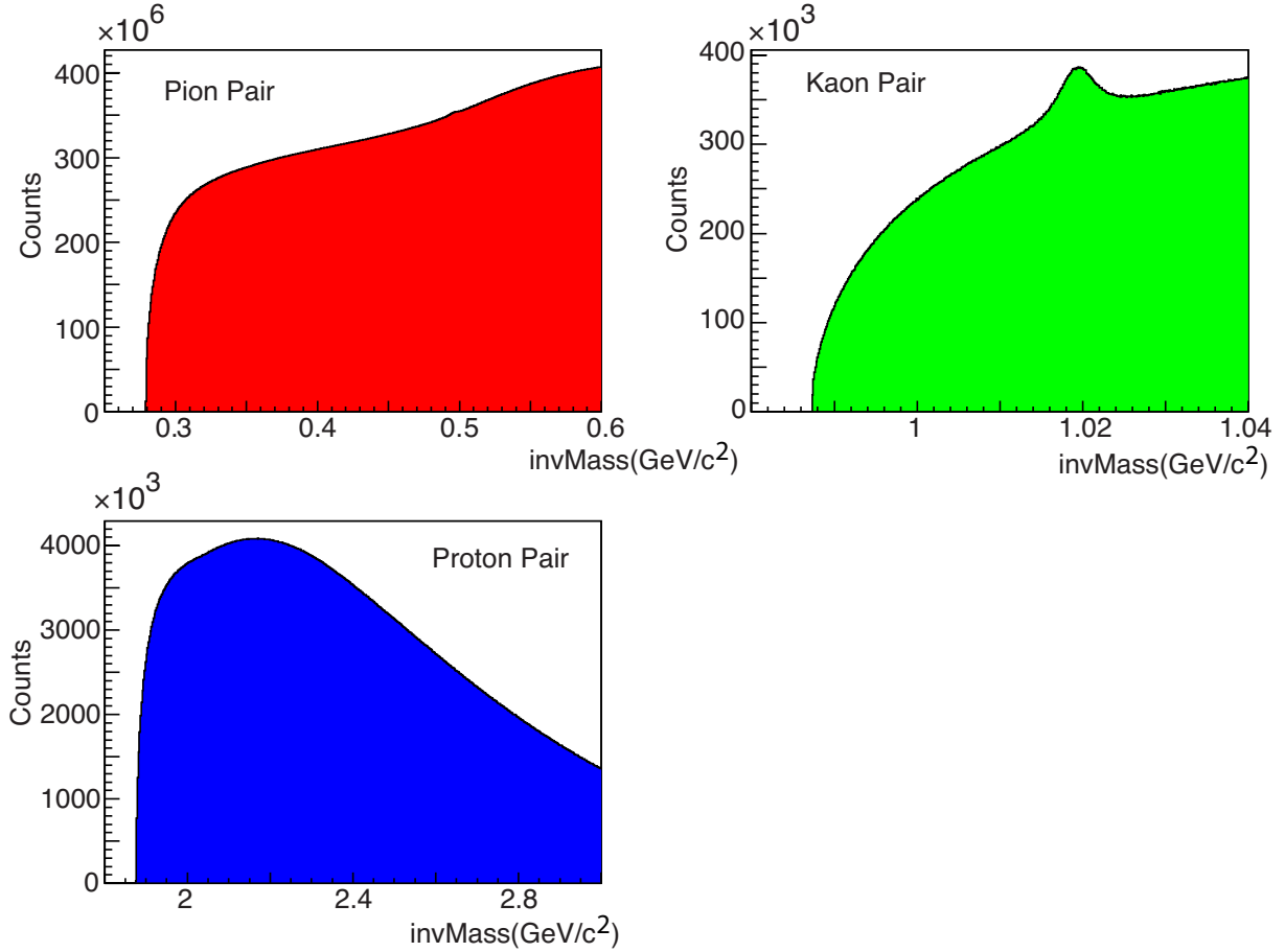
Figure 6.34: The invariant mass distribution of identified pion, kaon and proton pairs from STAR Run 10 Au+Au collisions at \sqrt{s_{NN}} = 200 GeV.
