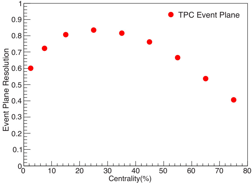
Figure 4.3: TPC event plane resolution for \sqrt{s_{\text{NN}}} = 200 GeV Au+Au MinBias collisions.
