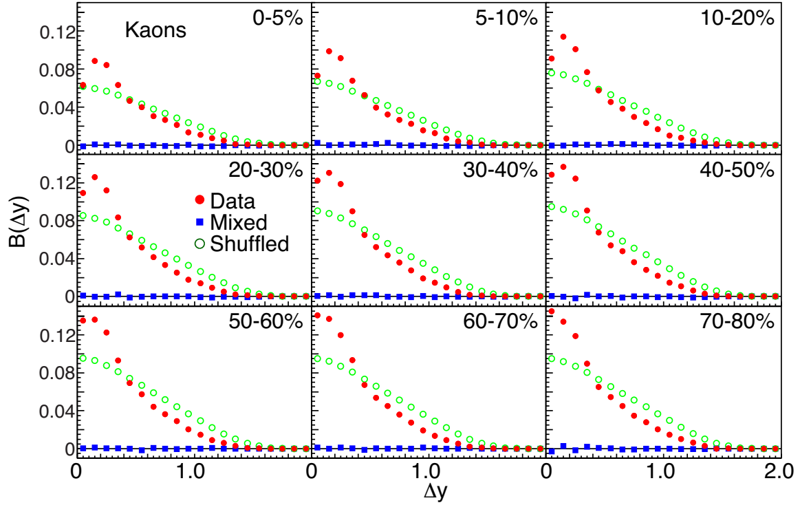
Figure 6.33: The balance function in terms of \Delta y for identified charged kaon pairs from STAR Run 10 Au+Au collisions at \sqrt{s_{\text{NN}}} = 200 GeV for nine centrality bins.
