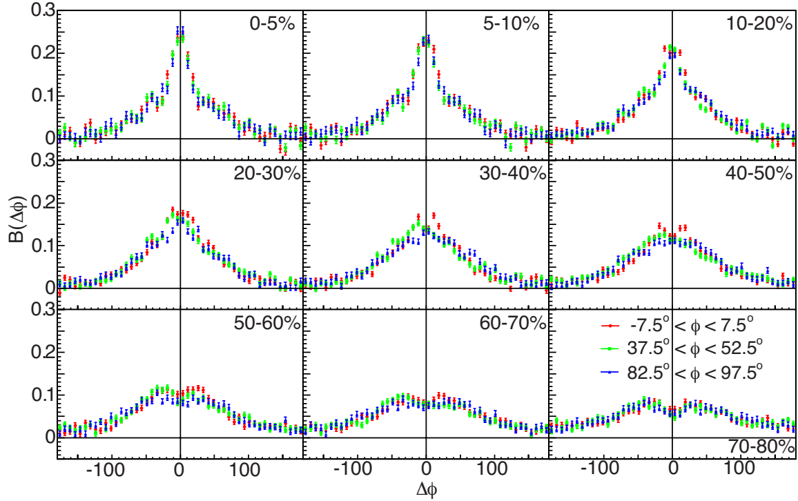
Figure 6.29: The balance function for \phi = 0^\circ (in-plane), \phi = 45^\circ , and \phi = 90^\circ (out-of-plane) particles pairs (not corrected for event plane resolution). Nine centralities bins are shown.
