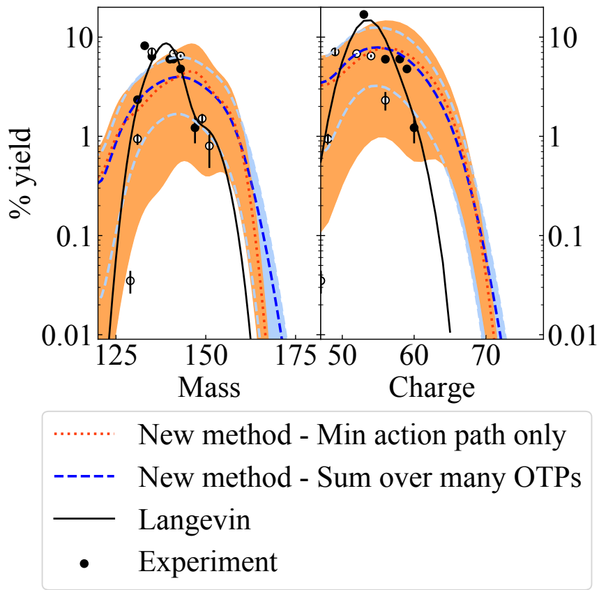
Figure A.2: PES and yield distribution for spontaneous fission of ^{240}\text{Pu} . On the left, the stars in the PES indicate outer turning points which were used to compute the cumulative yields. On the right, the black curve in the yields corresponds to the Langevin result, and experimental data comes from [4, 5].
