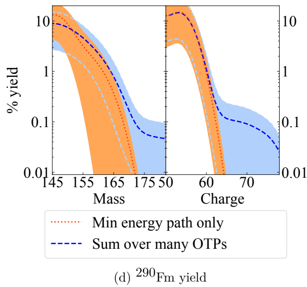
Figure 6.4: Similar to Figure 6.3, but for ^{290}\text{Fm} .
