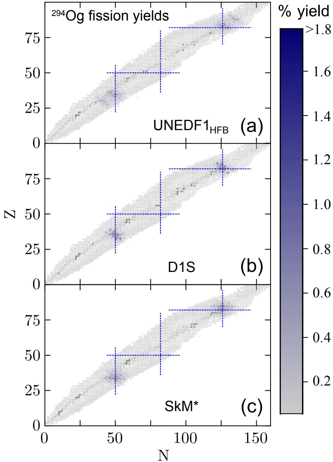
Figure 5.4: Fission fragment distributions for ^{294}\text{Og} obtained in UNEDF1 HFB (a), D1S (b), and SkM* (c) EDFs using the non-perturbative cranking ATDHFB inertia and the baseline dissipation tensor \eta_0 = (\eta_{11}, \eta_{22}, \eta_{12}) = (50\hbar, 40\hbar, 5\hbar) . Known isotopes are marked in gray [119]. Magic numbers 50, 82, and 126 are indicated by dotted lines.
