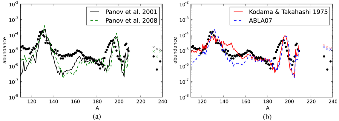
Figure 6.2: Final abundance patterns from four different simulations of neutron star merger ejecta, each using a different model for the fission fragment yields. The results are presented in two graphs solely for visual clarity. The dots represent the known solar r-process abundance pattern. Figure from [3].
