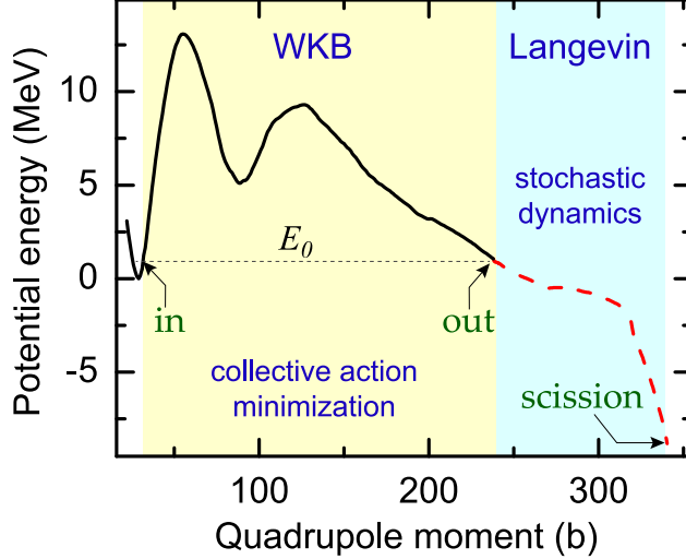
Figure 2.2: Schematic overview of the Langevin framework for fission calculations used in this dissertation. Figure from [64].
