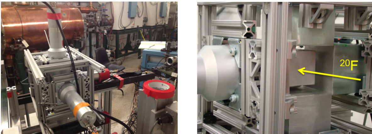
Figure 4.7: On the left the PVT set up can be seen. The rail the detector sits on and the optical fibers (the black cords) can be seen. On the right the CsI(Na) set up can be seen. In the center the implantation detector is seen.
