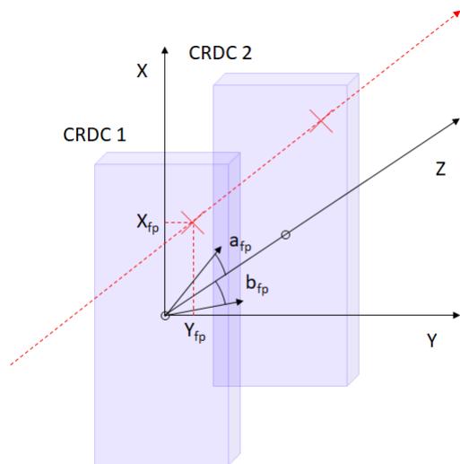
Figure 3.4: A schematic of the CRDC detectors used in the S800 focal plane and the position and angular information of the ion. The beam axis z , dispersive axis x , and non-dispersive axis y are shown. The first CRDC provides a measurement of the x and y position at the focal plane, x_{fp} and y_{fp} . The angle information a_{fp} and b_{fp} comes from the difference in the x and y positions between the two CRDC's.
