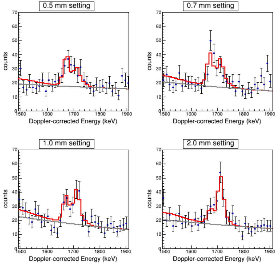
Figure 4.22: Doppler-corrected energy spectra of gamma rays from ^{20}\text{O} in each of the the three-foil, short-separation settings. A gate has been placed on the gamma-ray emission angle \theta < 50^\circ . The solid red lines are the results of a G4Lifetime simulation assuming a lifetime of \tau(2_1^+) = 16 ps and no feeding from the 4_1^+ state. The solid gray lines are exponential backgrounds fit to a large energy region.
