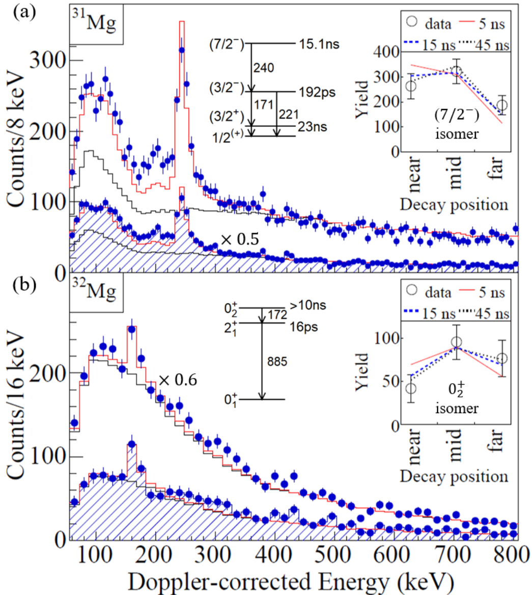
Figure 4.23: Doppler-corrected gamma-ray energy spectra are shown for data (blue circles), background from the scaled response of reaction products excluding the Mg isotopes (black lines), and the sums of the simulated and background responses (red lines). ^{31}\text{Mg} is shown (a) in the upper spectra and the constraint that the 244-keV transition only interacts within r = 20 mm of its first interaction is included in the lower, filled spectrum (scaled by 0.5). ^{32}\text{Mg} is shown (b) with the r = 20 mm gate applied to the 170-keV gamma ray in the upper spectrum (scaled by 0.6) and with additional gates requiring proper identification of the interaction points of the 885-keV gamma ray in the lower, filled spectrum. Insets show the number of decays near (250 to 525 mm), at mid-distance (525 to 700 mm) and far from the target (700 to 1000 mm). The data (open circles) is compared to simulations assuming lifetimes of 5 ns (red solid line), 15 ns (blue dashed line), and 45 ns (black dotted line).
