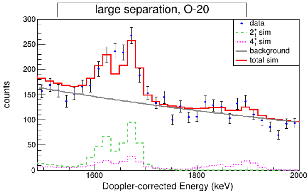
Figure 4.20: Doppler-corrected energy spectra of gamma rays from ^{20}\text{O} in the three-foil, large-separation setting. The data shows contributions at 1674-keV from the decay of the 2_1^+ state and at 1898-keV from the 4_1^+ state. The contributions of the populations of the 2_1^+ state and the 4_1^+ state are estimated with the simulated responses depicted with the dashed green and the dotted purple lines respectively. The solid gray line is an exponential background and the solid red line is the sum of the two simulation components and the background.
