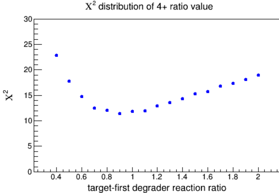
Figure 4.10: \chi^2 distribution for the ratio of the number of reaction on the target to those on the first degrader for the 4_1^+ state of ^{32}\text{Mg} . A clear minimum is visible at r(4_1^+) = 0.9(2) .
