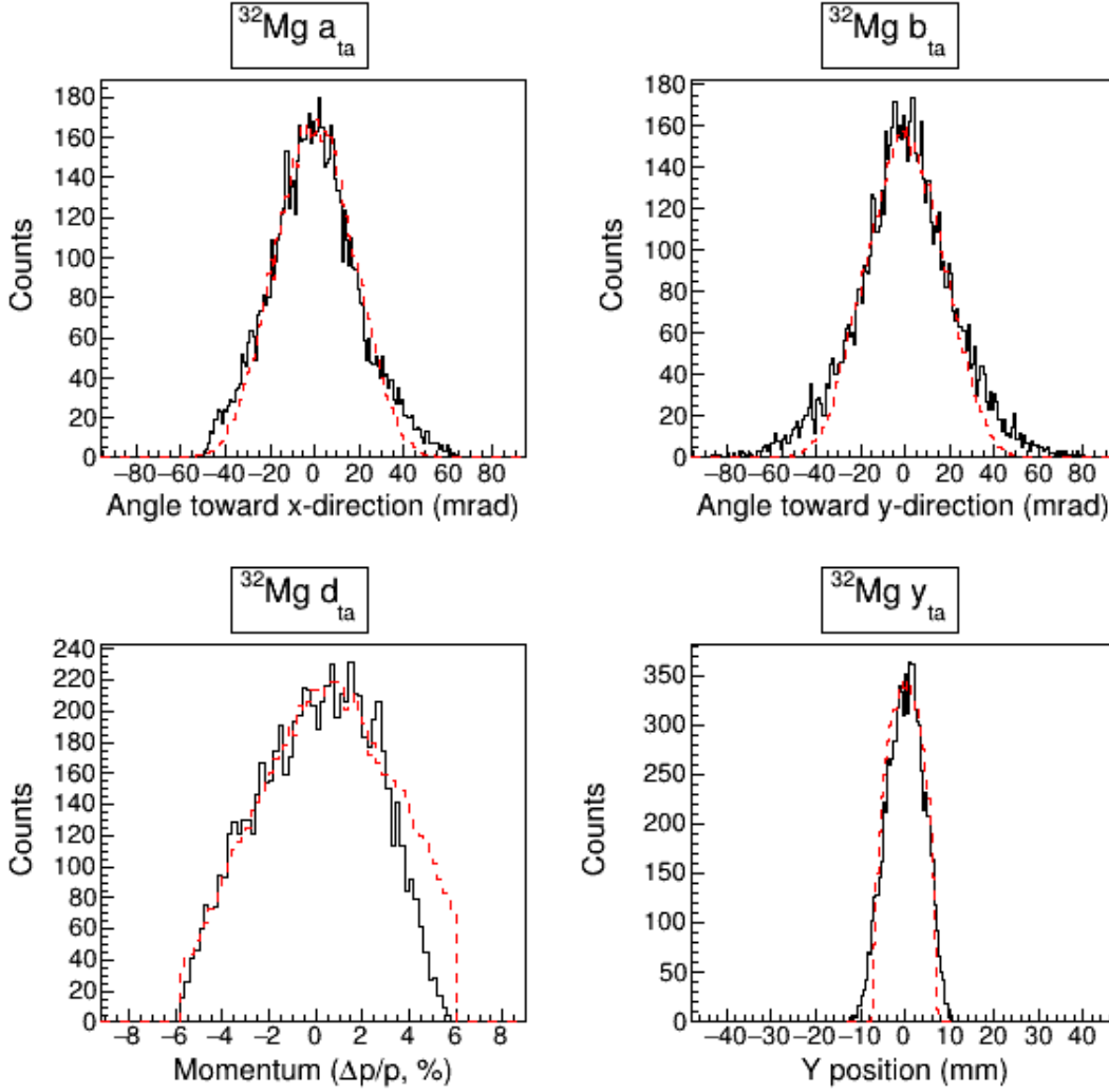
Figure 4.3: The a_{ta} , b_{ta} , d_{ta} and y_{ta} distributions of ^{32}\text{Mg} . Data is shown as a solid black line and a scaled simulation is shown as a dashed red line.
