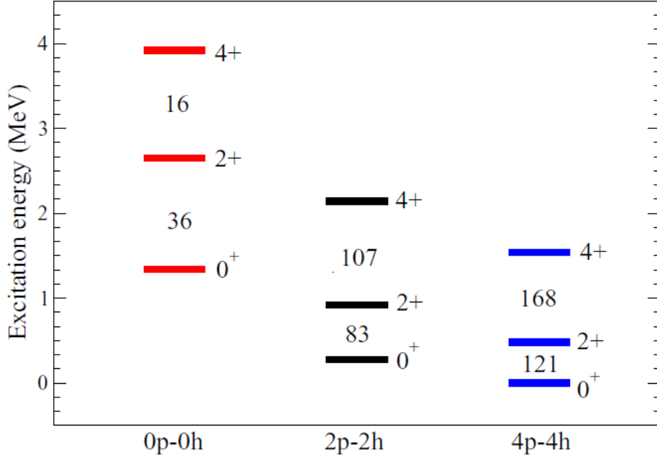
Figure 5.3: The 0^+ , 2^+ , and 4^+ states and B(E2) values in ^{32}\text{Mg} from the SDPF-U-MIX calculation with fixed npnh configuration. Figure is from Ref. [21]. The numbers between the states represent the B(E2) value of that transition in e^2\text{fm}^4 .
