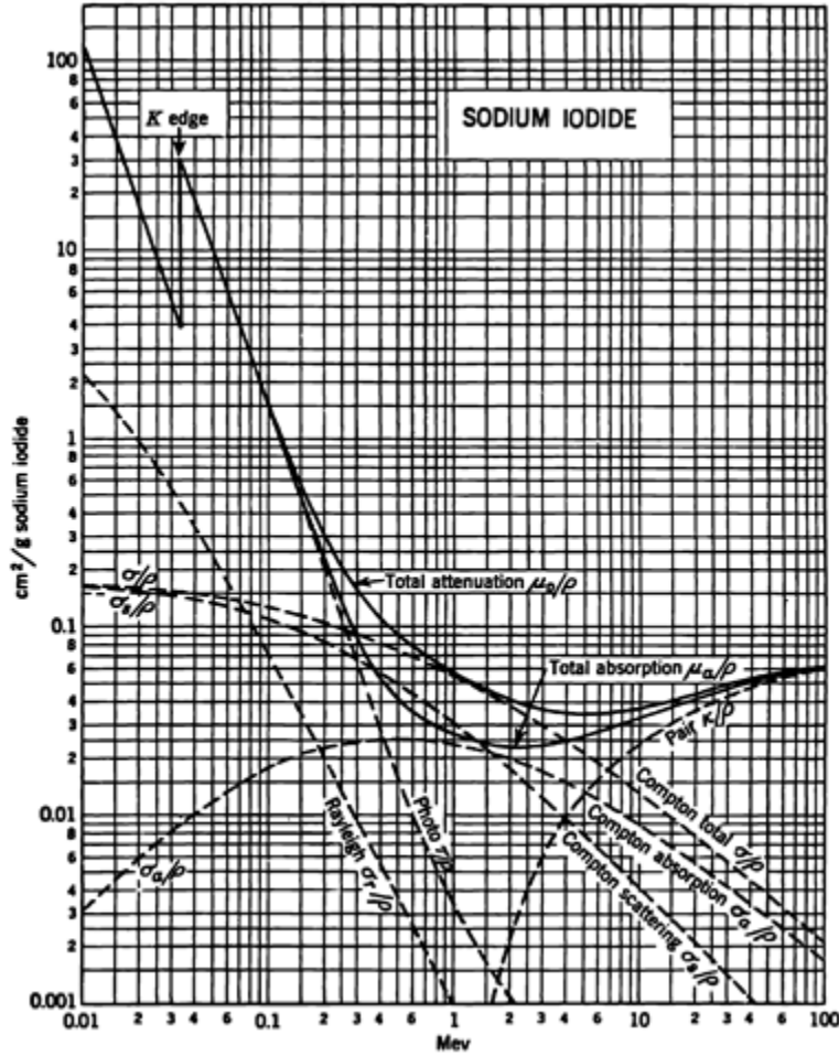
Figure 2.1: The mass attenuation coefficients for gamma-ray interactions in sodium iodide. Photoelectric absorption, Compton scattering and pair production interactions account for nearly all of the attenuation. The figure is from Ref. [48].
