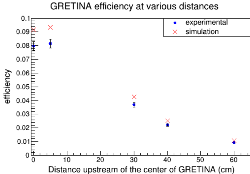
Figure 3.14: The efficiency of GRETINA for the 779-keV gamma ray from a ^{152}\text{Eu} radioactive source placed at various distances upstream of the center of GRETINA. The measured efficiency is shown with blue circles and error bars and the efficiency of GRETINA in the GEANT4 simulation is shown as red saltire ( \times ) symbols.
