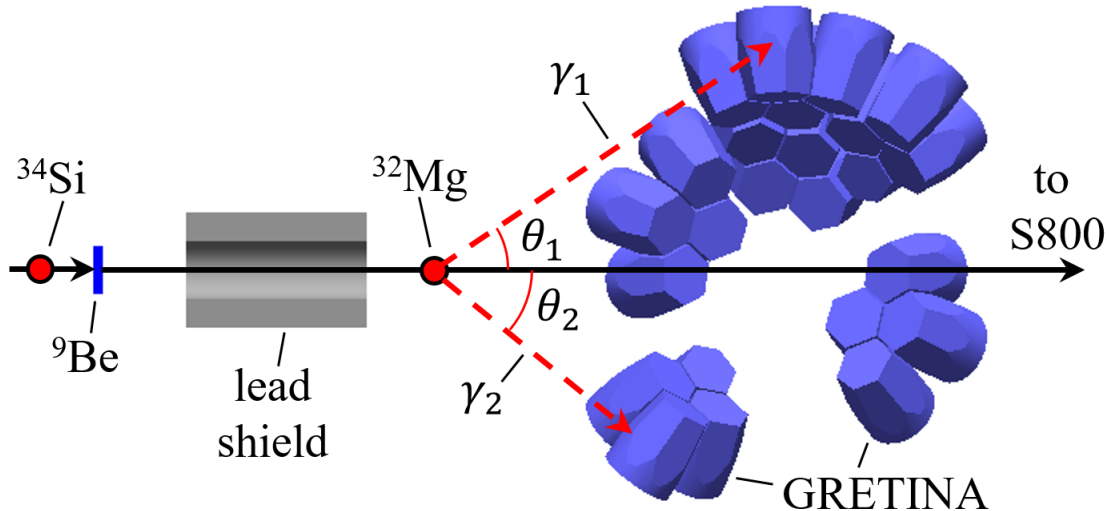
Figure 3.20: The setup for the part of the experiment with the upstream target, designed to measure the 0_2^+ isomer of ^{32}\text{Mg} . The ^9\text{Be}(^{34}\text{Si}, ^{32}\text{Mg})X reaction populates the 0_2^+ isomer which emits a cascade of gamma rays \gamma_1 and \gamma_2 at angles \theta_1 and \theta_2 relative to the ion trajectory.
