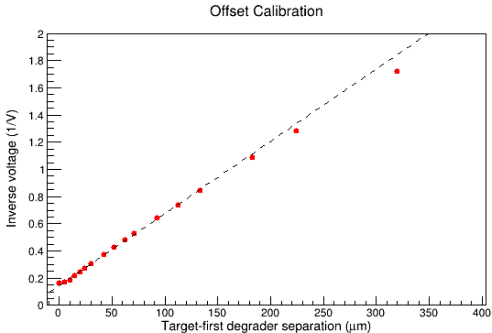
Figure 3.19: The inverse of the induced voltage on the target foil at various separations from the first degrader. The separation is measured relative to the location where the induced voltage saturated, indicating electric contact between the foils. The change in separation is measured by the motor displacement. The red dots are data points which are fit with a linear function shown by a black dotted line. The fit matches the data well for separation < 150 \mu\text{m} but deviates somewhat at larger separation. At large separation the assumption that the foils behave like a parallel-plate capacitor breaks down and the induced voltage value changes by small degrees that are difficult to resolve.
