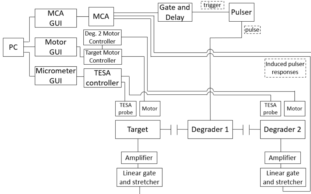
Figure 3.18: A diagram showing the connections between the TRIPLEX systems and the PC. The PC uses the multi-channel analyzer (MCA) GUI, the Motor GUI, and the Micrometer GUI to access the three systems represented here. The Pulser sends a trigger to the MCA and a pulse to Degradation 1 which causes induced pulse responses on Target and Degradation 2 due to the capacitance with these foils. NIM modules are used to manipulate the trigger signal and the induced pulse responses. A motor controller operates and reads the displacement value from each motor. The TESA controller reads the measurements from the TESA micrometers.
