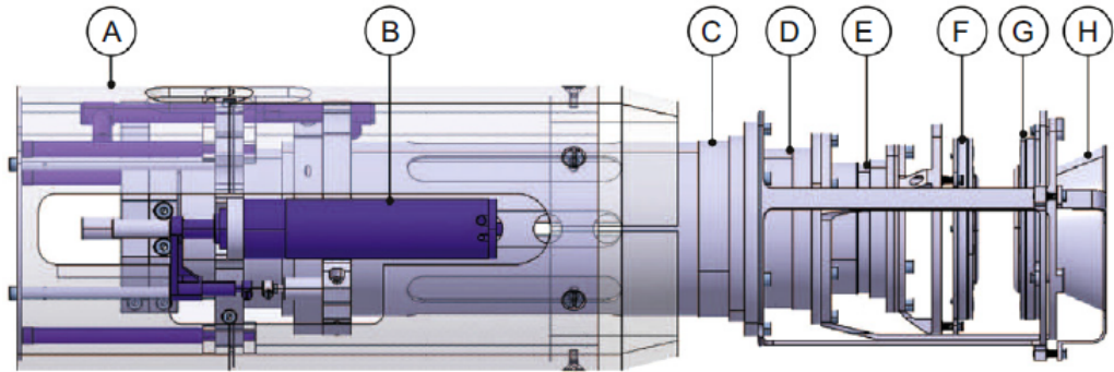
Figure 3.15: The TRIPLEX device used in this experiment. The schematic shows (A) the outer casing, (B) a piezoelectric motor, (C) the outermost tube, (D) the middle stationary tube, (E) the innermost tube, (F) the target positioned by the innermost tube E, (G) the first degrader held stationary by the middle tube, and (H) the second degrader positioned by the outermost tube. The figure is from Ref. [81].
