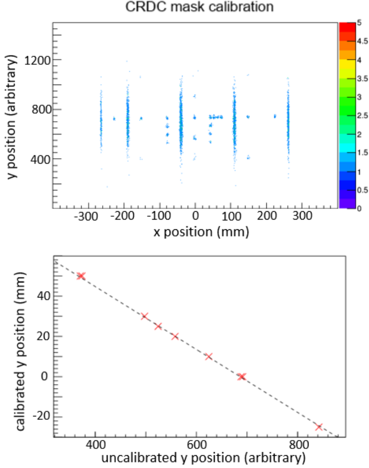
Figure 3.6: The top section shows the uncalibrated x and y positions of the first CRDC with the mask placed in front. The holes in the mask allow ions to pass through to the CRDC. The lower section shows the linear calibration between the raw position values ch and the calibrated positions y . The line is defined by y = -0.156248ch + 107.28
