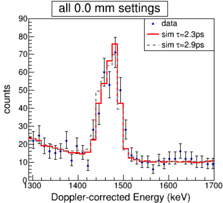
Figure 4.17: Doppler-corrected energy spectra of gamma rays from ^{30}\text{Mg} in the three-foil, short-separation setting. A gate was placed on the gamma-ray emission angle \theta < 50^\circ . The solid red line depicts the simulation results assuming a lifetime of 2.3 ps. The dashed gray line corresponds to a simulation with a lifetime of 2.9 ps.
