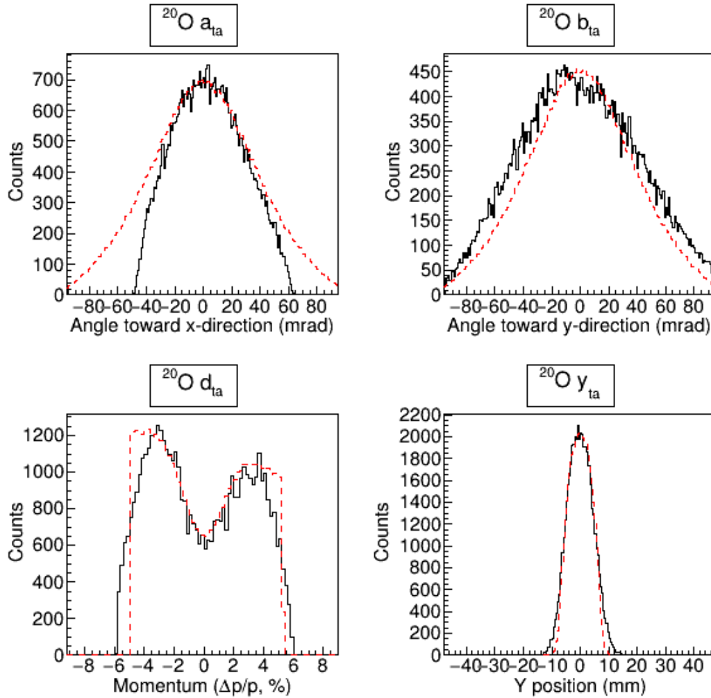
Figure 4.19: The a_{ta} , b_{ta} , d_{ta} and y_{ta} distributions of the ^{20}\text{O} reaction product in the three-foil settings. Data is shown as a solid black line and a scaled simulation is shown as a dashed red line.
