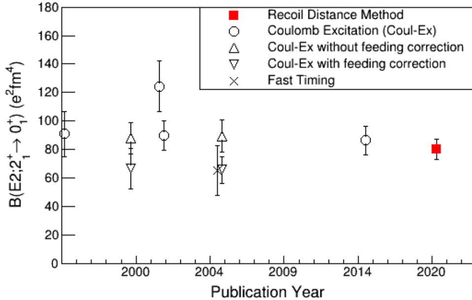
Figure 5.1: The B(E2; 2_1^+ \rightarrow 0_1^+) value in ^{32}\text{Mg} reported in experiments over the past 25 years. The present RDM measurement is shown with a red square. The Coulomb-excitation measurements from Refs. [13,37,38,40] are shown with open circles. The open triangles are the results from Refs. [36,39]. The upward-pointing triangles reflect the B(E2) values without feeding corrections while the corresponding downward-pointing triangles take into account feeding corrections. The saltire symbol ( \times ) represents the fast timing measurement of Ref. [41].
