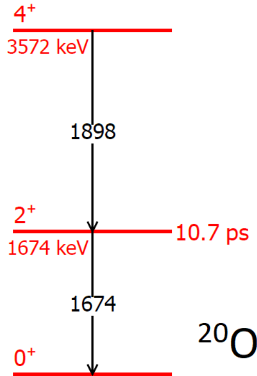
Figure 4.18: Partial level scheme of ^{20}\text{O} .
