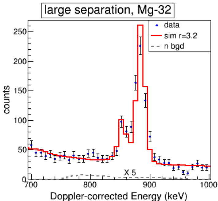
Figure 4.7: Doppler-corrected energy spectra showing the two components of the 885-keV peak in the large separation setting. Only gamma rays observed in the laboratory frame with an emission angle of \theta < 70^\circ are shown. The solid red line depicts the result of a G4Lifetime simulation that assumes a ratio of r(2_1^+) = 3.2 for the number of reactions on the target divided by the number of reactions on the first degrader that populate the 2_1^+ state of ^{32}\text{Mg} . The dashed gray line is the background contribution from the neutron-induced 1014-keV gamma ray from ^{27}\text{Al} and it is scaled by \times 5 in this image.
