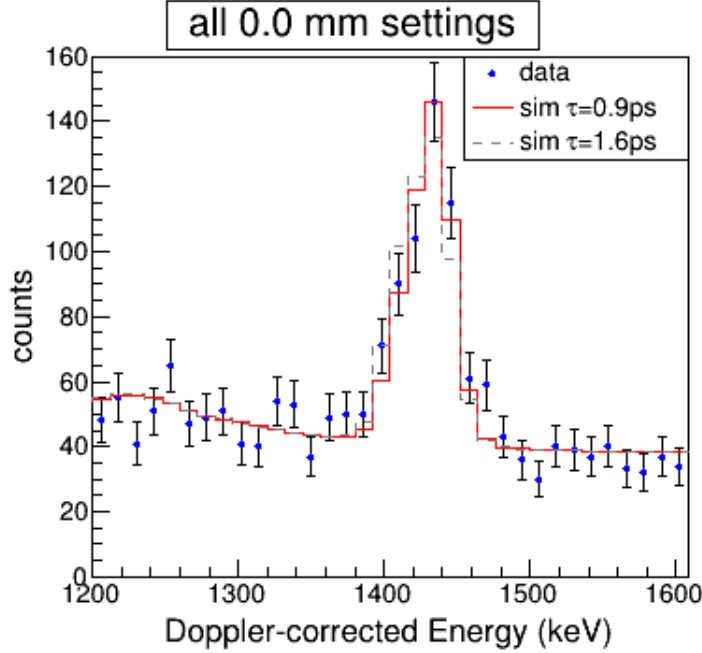
Figure 4.14: Doppler-corrected energy spectra showing the lineshape of the 1437-keV transition. The solid red line depicts the results of GEANT4 simulations that assume a lifetime of 0.9 ps for the 2_1^+ state of ^{32}\text{Mg} , while the grey dashed line assumes a lifetime of 1.6 ps.
