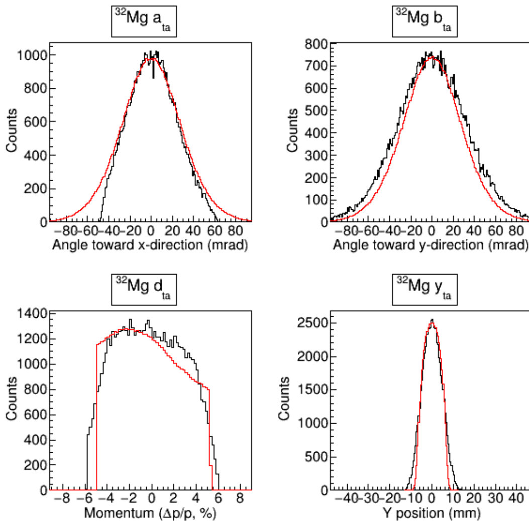
Figure 3.22: The a_{ta} , b_{ta} , d_{ta} and y_{ta} distributions of the ^{32}\text{Mg} reaction product with all three foils installed in the TRIPLEX device. Data is shown as a black line and a scaled simulation is shown as a red line.
