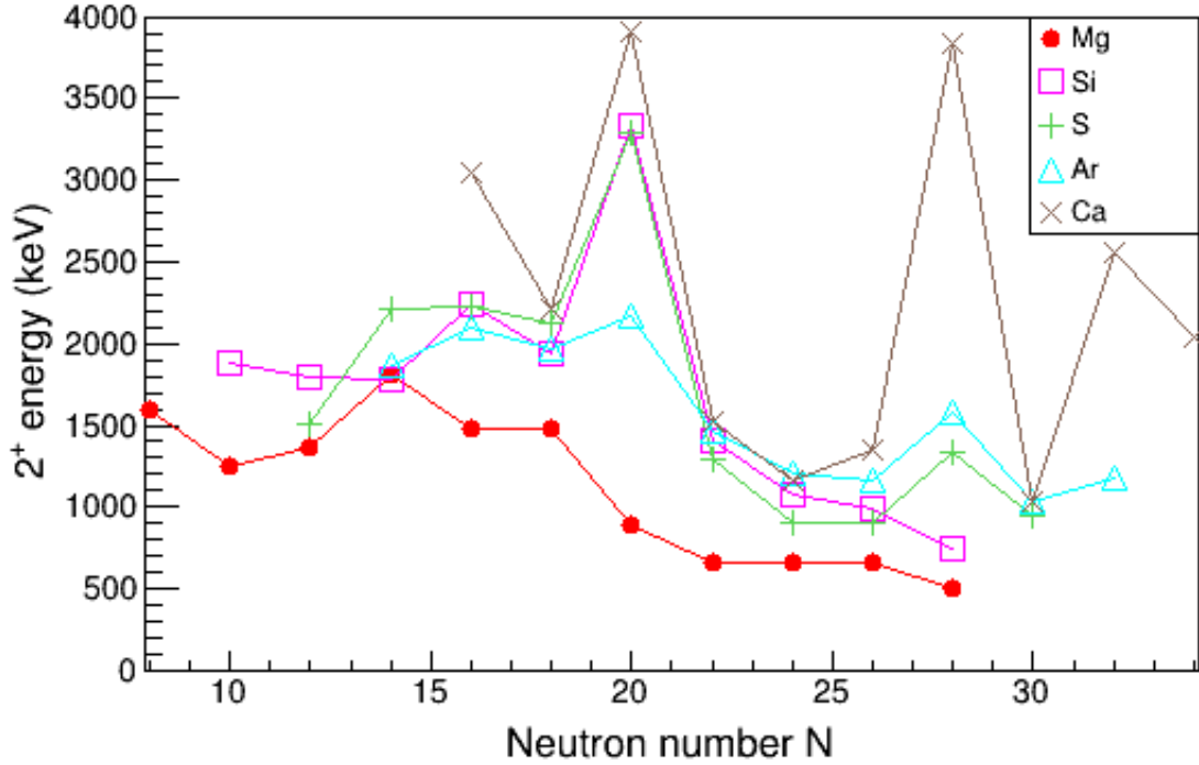
Figure 1.6: The energy of the first 2^+ states in even-even nuclides. For many nuclides with the magic number N = 20 or N = 28 the first 2^+ energy is larger than the neighboring even-even isotopes. This is not the case for ^{32}\text{Mg} at N = 20 and for ^{40}\text{Mg} and ^{42}\text{Si} at N = 28 .
