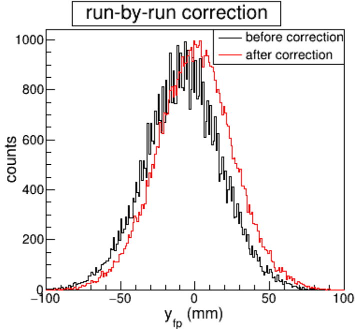
Figure 3.11: y_{fp} distributions, gated on ^{32}\text{Mg} reaction products. The distribution before run-by-run corrections is shown in black, while the distribution after run-by-run corrections is shown in red. The correction causes the distribution to be centered in the CRDC and slightly narrower.
