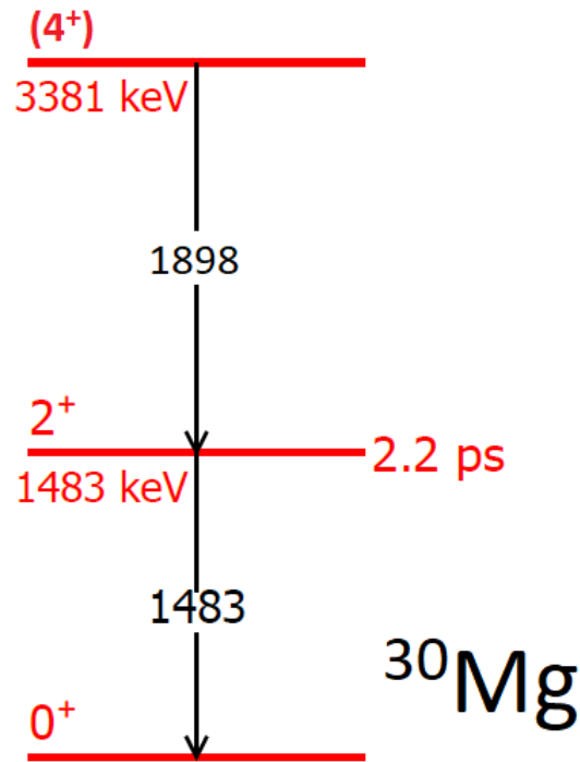
Figure 4.15: Partial level scheme of ^{30}\text{Mg} .
