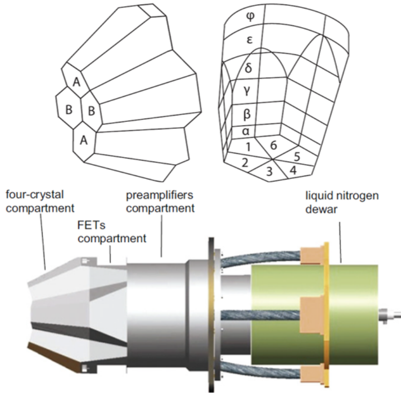
Figure 3.12: Diagram of a GREY module. The full module is shown in the bottom section. The four high-purity germanium crystals in a single module are depicted in the top-left. The segmentation of a single crystal is depicted in the top-right. The figure is adapted from Ref. [67].
