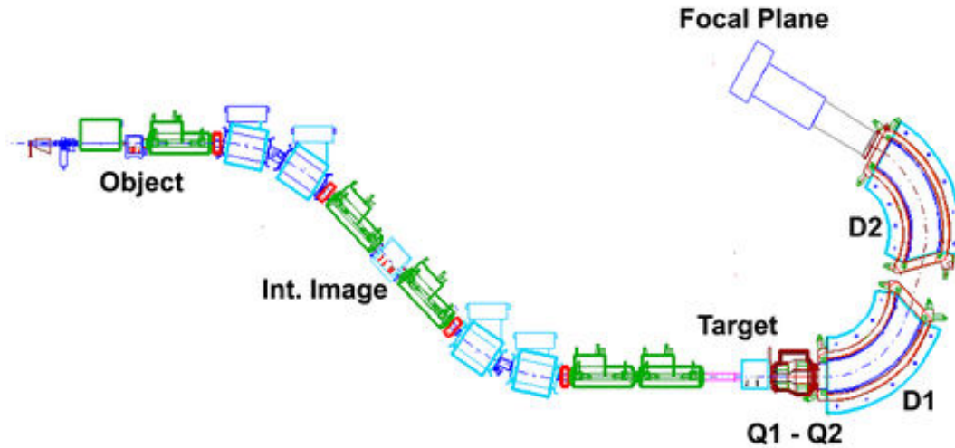
Figure 3.1: A schematic of the S800 spectrograph. The figure is from Ref. [71].
