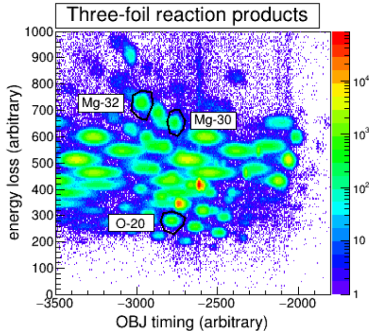
Figure 4.6: The PID for reaction products resulting from the ^{34}\text{Si} secondary beam and the ^9\text{Be} target in the three-foil settings. The x -axis is the TOF in arbitrary units between the E1 and OBJ scintillators of the S800 spectrograph. The y -axis is the energy loss of ions traveling through the ionization chamber in arbitrary units. The software gates used to select the ^{32}\text{Mg} , ^{30}\text{Mg} , and ^{20}\text{O} reaction products are shown with solid black lines.
