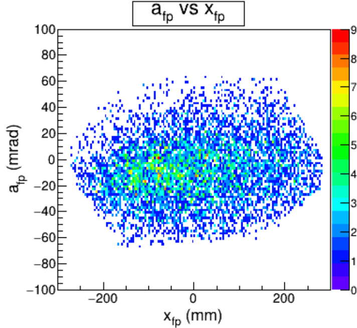
Figure 4.25: Distribution of the angle a_{fp} and the position x_{fp} for ^{32}\text{Mg} reaction products in the target-only setting with the TRIPLEX device. A portion of the ^{32}\text{Mg} reaction products are lost at the edges of the distribution with extreme values of both a_{fp} and x_{fp} .
