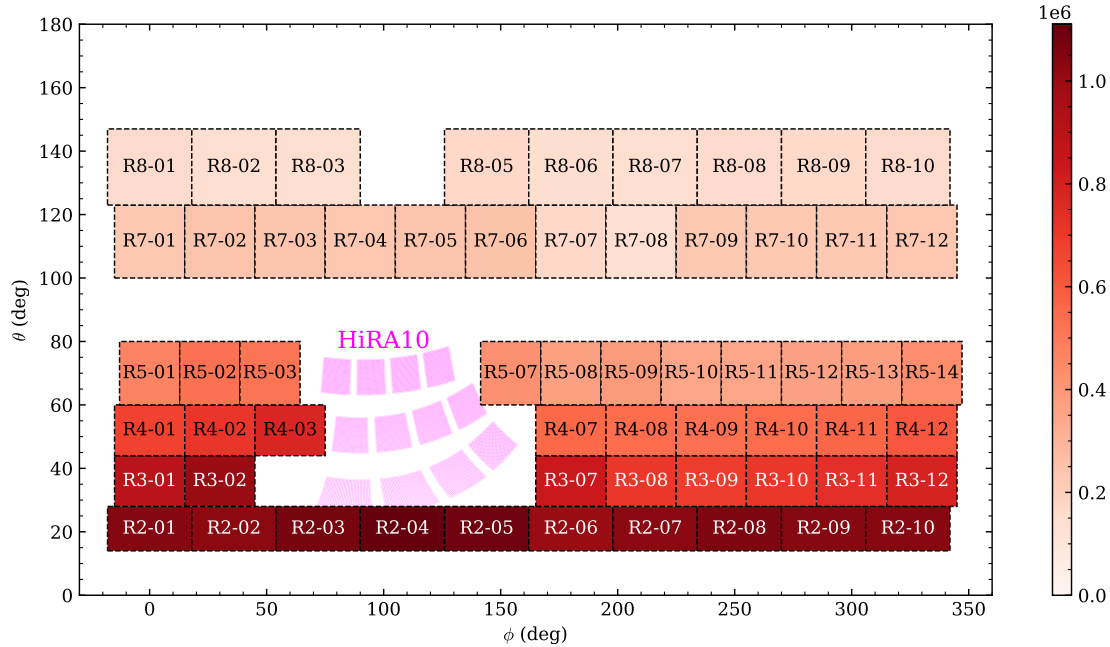
Figure 2.4 Microball hit pattern in run 4520. Each rectangle represents a scintillator. Ring number and scintillator number are labeled in the format of “ RX-Y ”, e.g. “R2-10” means scintillator 10 of Ring 2.
