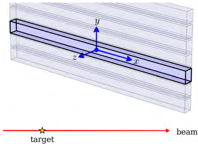
Figure 4.3 A schematic view of the NW bar coordinate system. The drawing is not to scale, however the relative sizes of the NW bar dimensions have been preserved. Excluding the Pyrex thickness, each bar has a dimension of 193.04 \text{ cm} \times 7.62 \text{ cm} \times 6.35 \text{ cm} ( x, y, z ).
